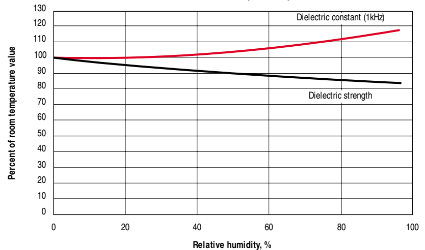
Figure 1 – EFFECT OF HUMIDITY ON ELECTRICAL PROPERTIES NOMEX® TYPE 414 – 0.25 MM (10MIL)
