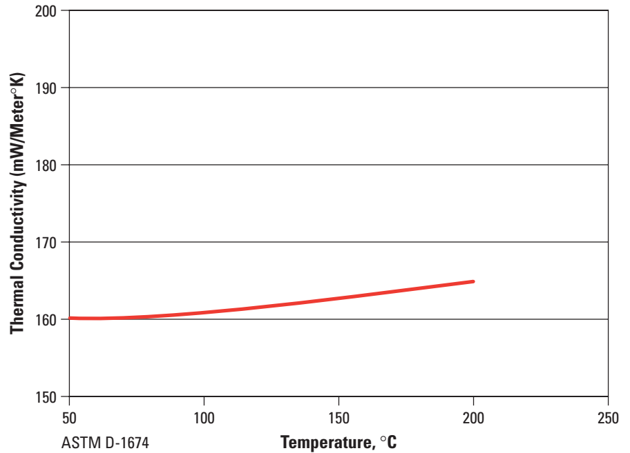
Figure 1 – THERMAL CONDUCTIVITY VS. TEMPERATURE 3.2 mm (125 mil) Type 994
