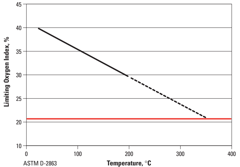
Figure 2 – LIMITING OXYGEN INDEX (LOI) 6.4 mm (250 mil) Type 994
